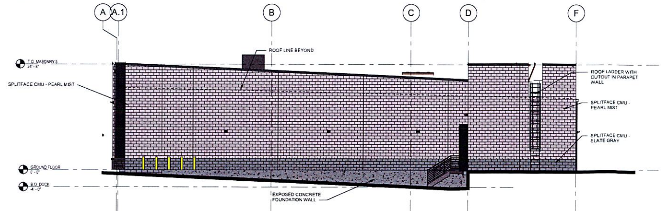
4 RIGHT ELEVATION (EAST) SCALE: 1/8" = 1'-0"
