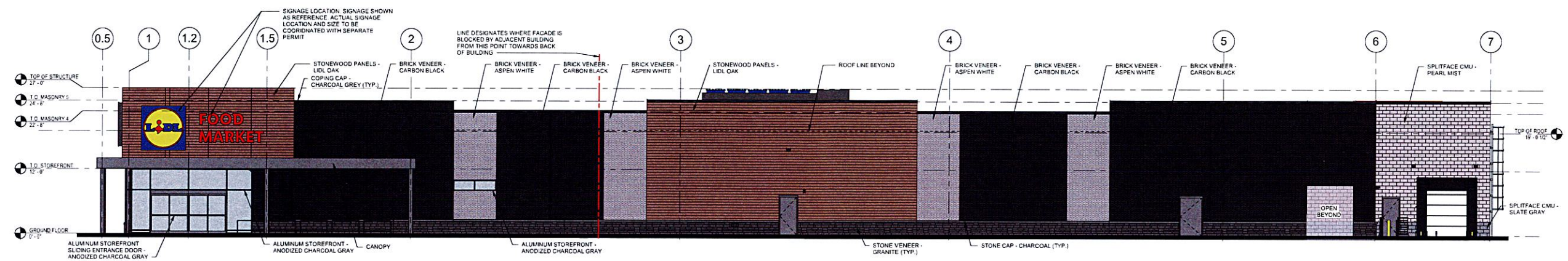
2 FRONT ELEVATION (SOUTH) SCALE: 1/8" = 1'-0"
