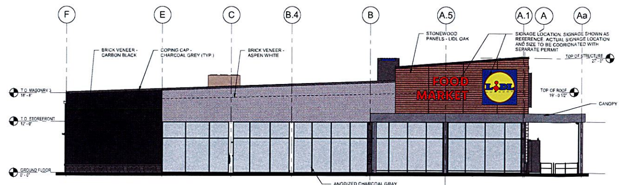
1 LEFT ELEVATION (WEST) SCALE: 1/8" = 1'-0"
