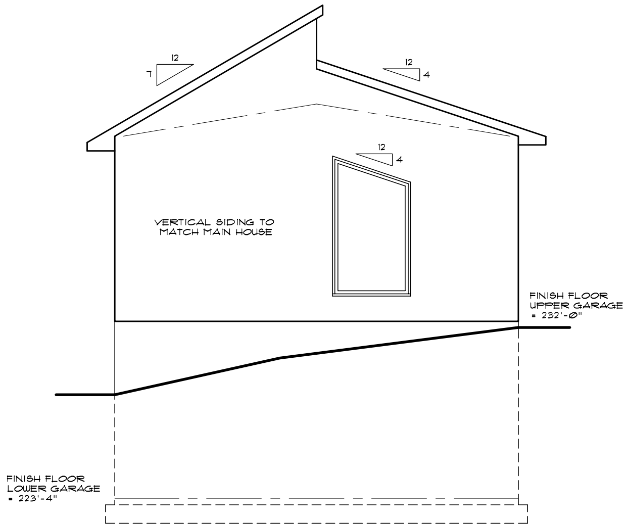
Elevation From Street Mandell Residence
