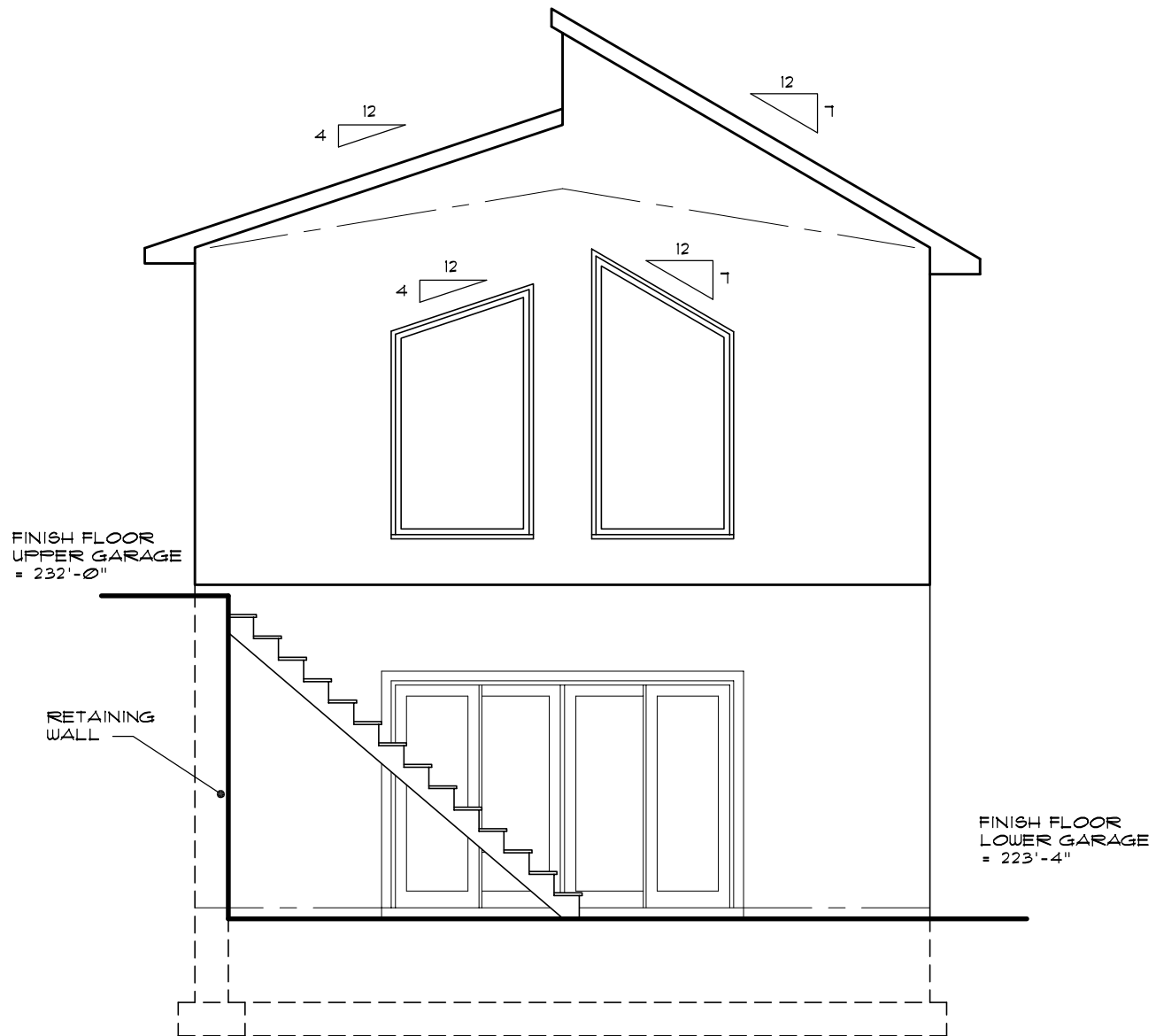
Elevation From River Mandell Residence
