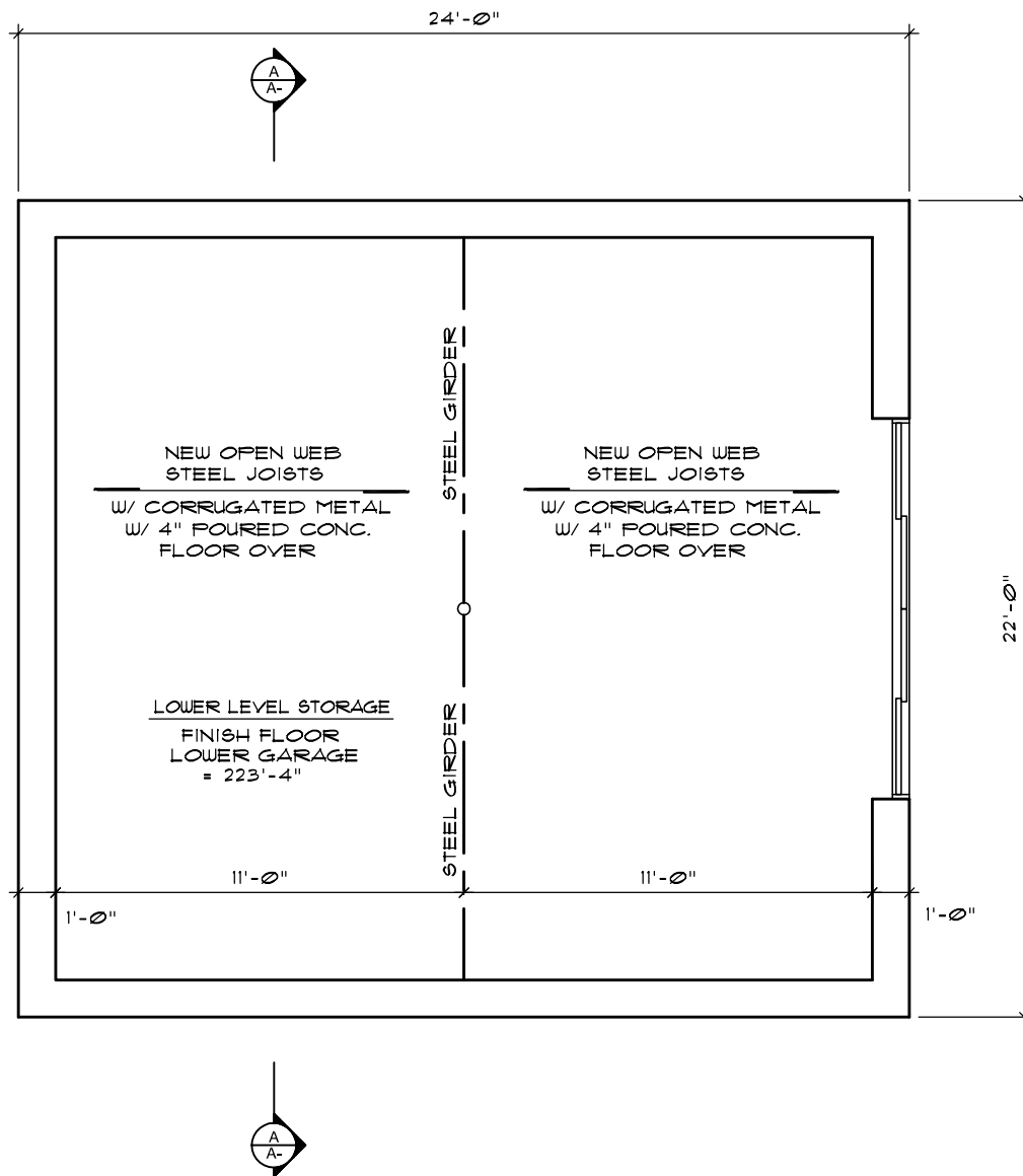
Lower Level Garage Plan Mandell Residence
