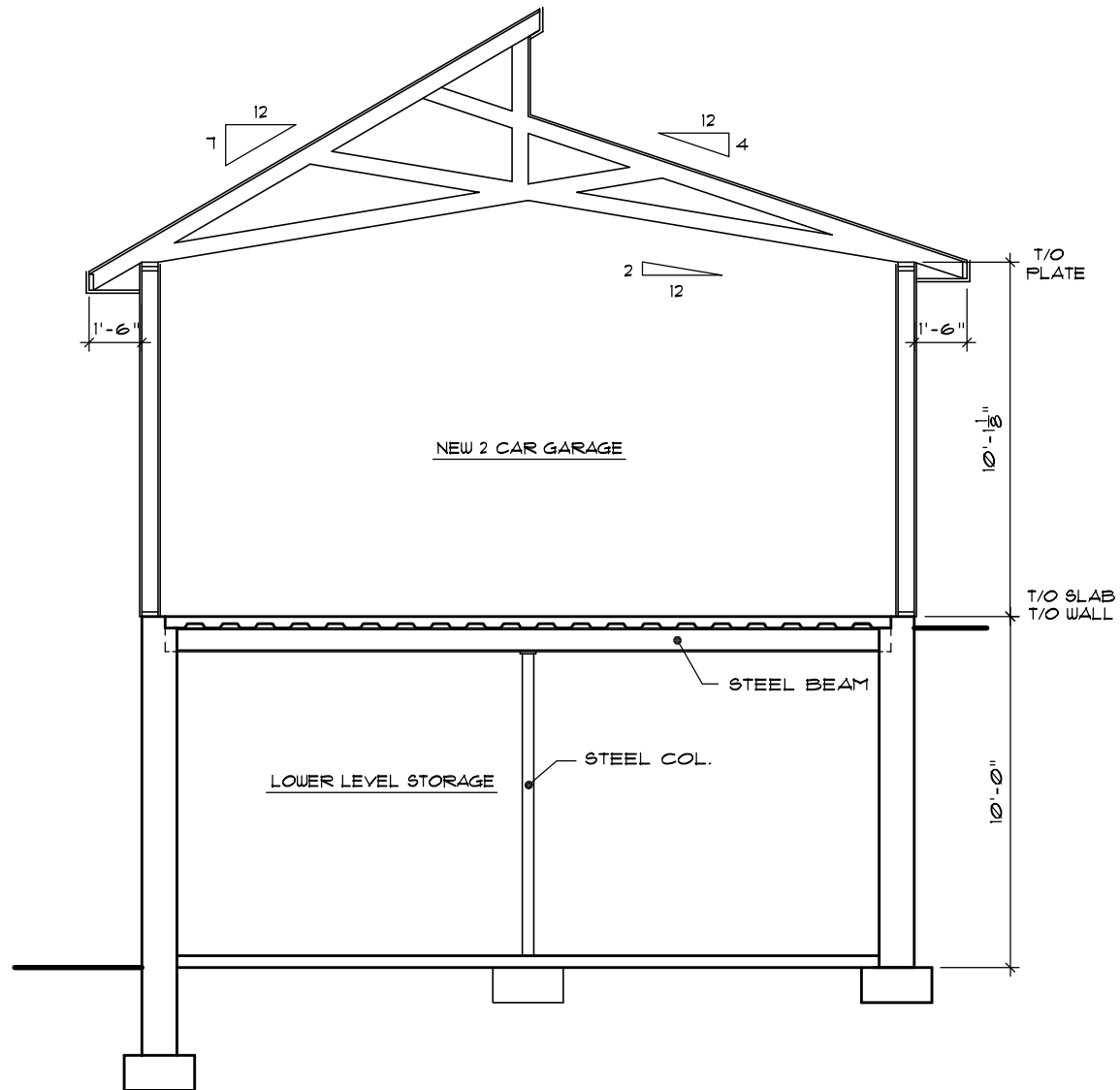
Building Section A-A Mandell Residence
